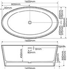
Size: 1600x750x600mm / 1600x900x580mm
