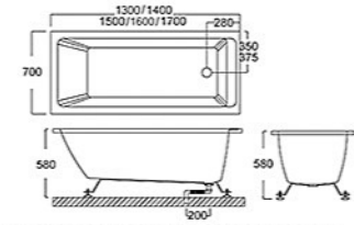
Size: 1300x700x580mm/1400x700x580mm Size: 1500x700x580mm/1600x700x580mm Size: 1700x700x580mm
